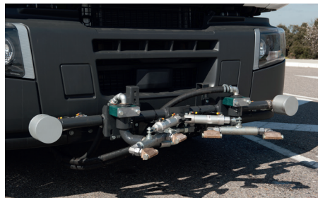
Washer spray cone and nozzle bar.
